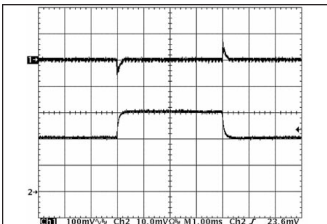
Figure 11: Output voltage response to step-change in load current (50%-75%-50% of I_{out(max)} ; dI/dt = 0.1\text{A}/\mu\text{s} ). Load cap: 15\mu\text{F} , 450\text{ m}\Omega ESR tantalum capacitor and 1\mu\text{F} ceramic capacitor. Top trace: V_{out} (100mV/div), Bottom trace: I_{out} (10A/div).
