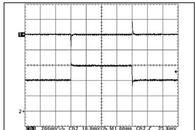
Figure 12: Output voltage response to step-change in load current (50%-75%-50% of I_{out(max)} ; dI/dt = 5\text{A}/\mu\text{s} ). Load cap: 480\mu\text{F} , 15\text{ m}\Omega ESR tantalum capacitor and 1\mu\text{F} ceramic capacitor. Top trace: V_{out} (200mV/div), Bottom trace: I_{out} (10A/div).
